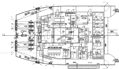
POOP DECK
