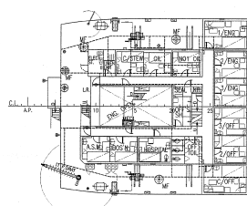
BOAT DECK
