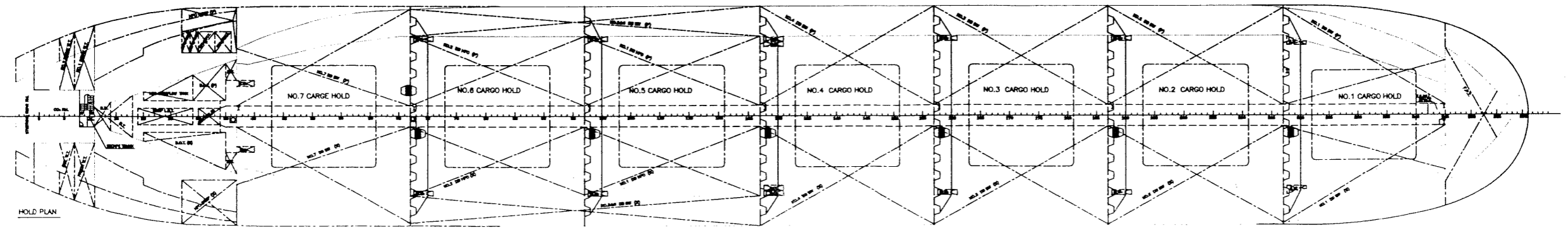
UPPER DECK
