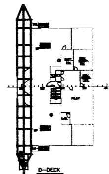
D-DECK
