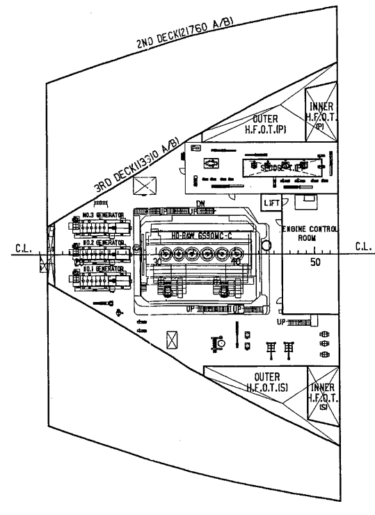
3RD DECK
