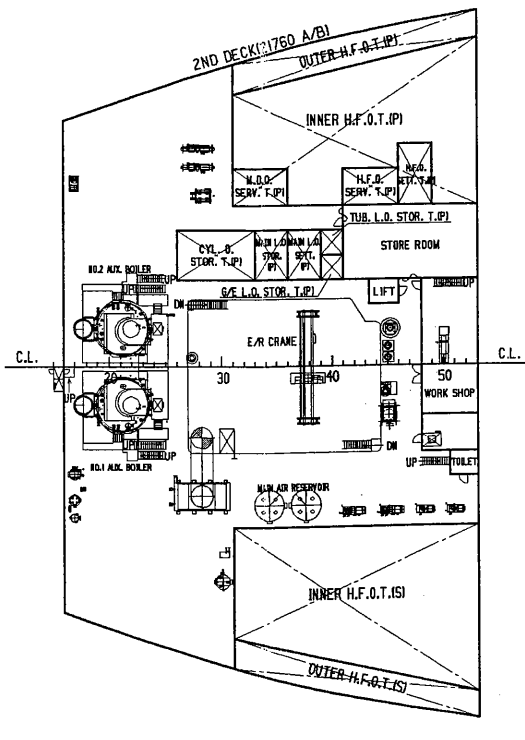
2ND DECK
