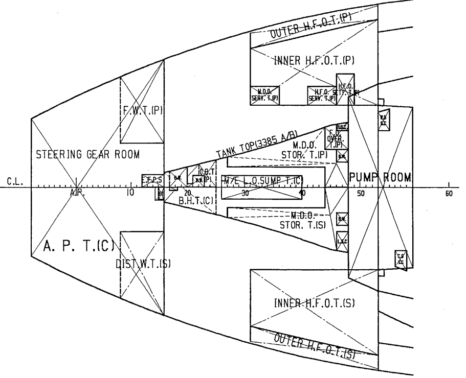
S/G & T/TOP
